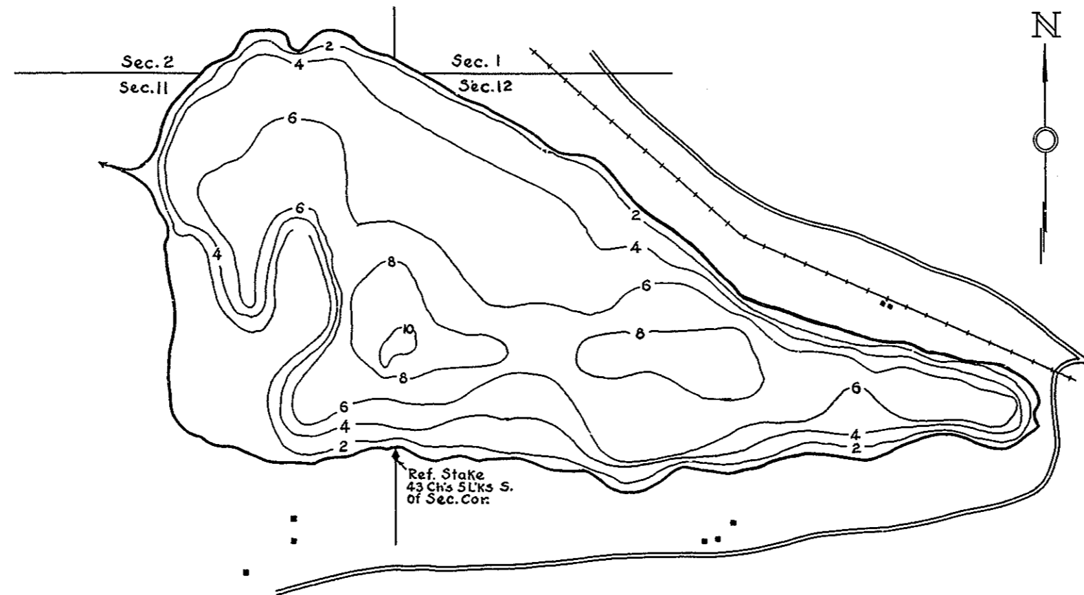
Contour Map Contour Interval - 2'
