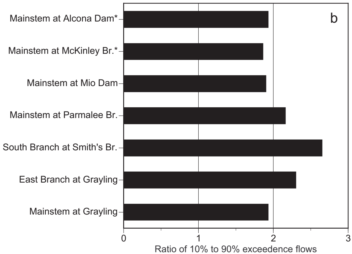
Figure 6.—Flow stability (expressed as the ratio of 10% and 90% exceedence flows) of: a) Michigan streams having catchments comparable in size to the Au Sable River below Foote Dam; and b) gauged Au Sable River catchments upstream of Mio. Data from United States Geological Survey. * indicates data for 1997 only.
