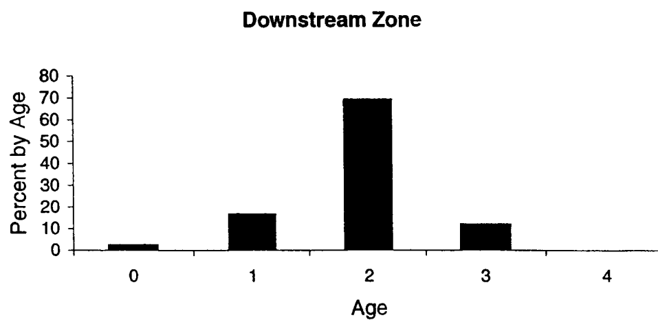
Figure 1.17. Rainbow trout age structure within each zone on the Pine River between 1996 and 1999.
