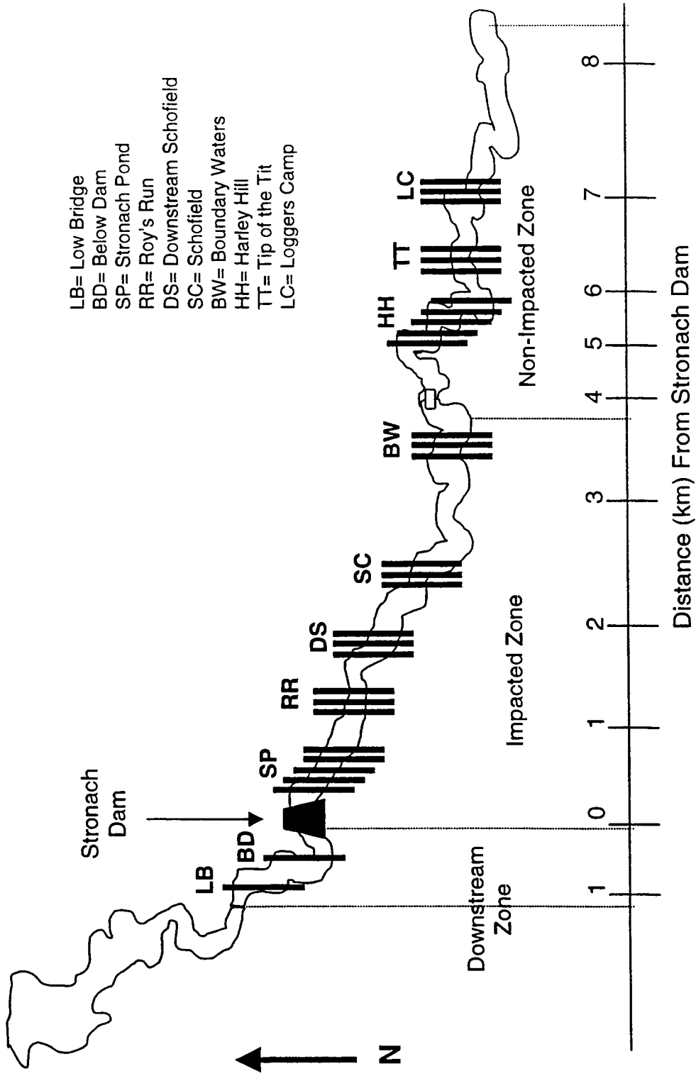
Figure 1.3. Cross-sectional survey sites located on the Pine River.
